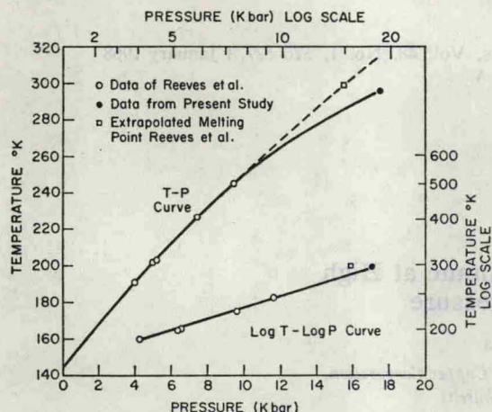
FIG. 1. T - P and \log T - \log P representations of the melting curve of n -pentane (solid curves). Dashed curve represents Simon relation proposed by Reeves et al. 2
